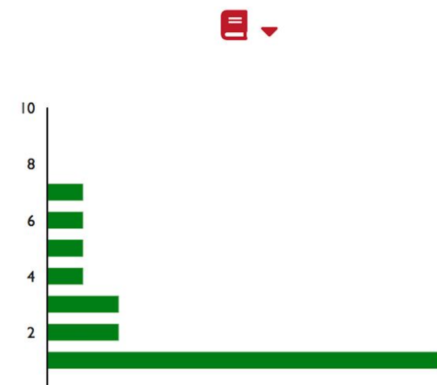
Top 10 co-hashtag
