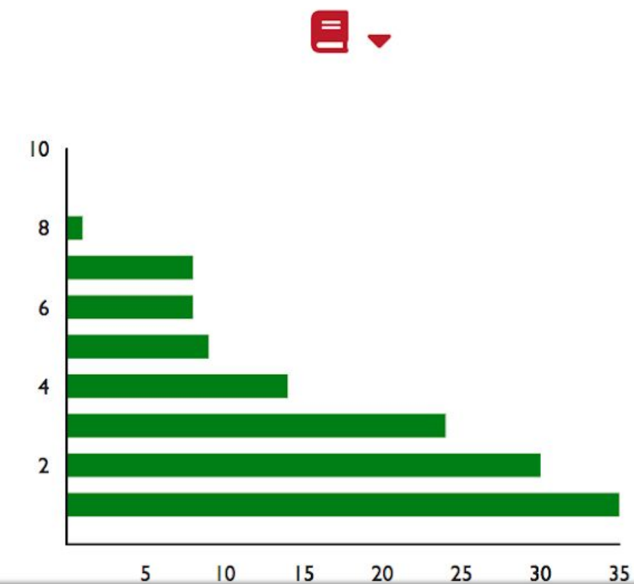
Top 10 Retweet
